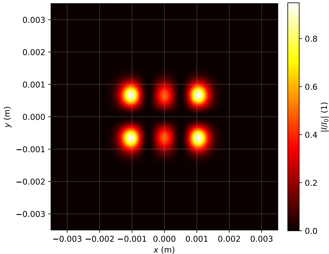
Intensity profile I(x, y, z = 1.672)/I_0 , P_{in}=2.0P_{cr} , artificial time
